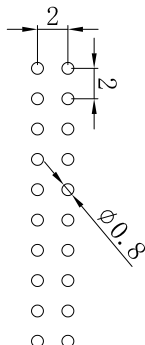
Recommended P.C.Board Layout
